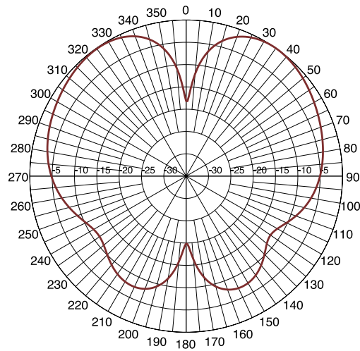
MLPV430 - Elevation
