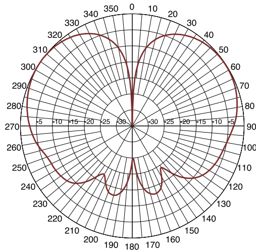
MLPV800 - Elevation
