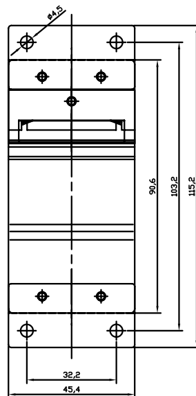
Backboard rear view (Mount kit)
